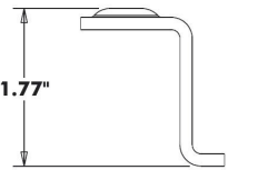
GV STEEL STIFFENER BAR END VIEW
