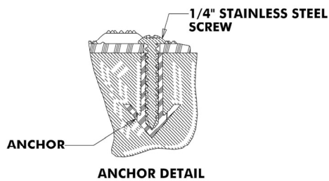
ANCHOR DETAIL
